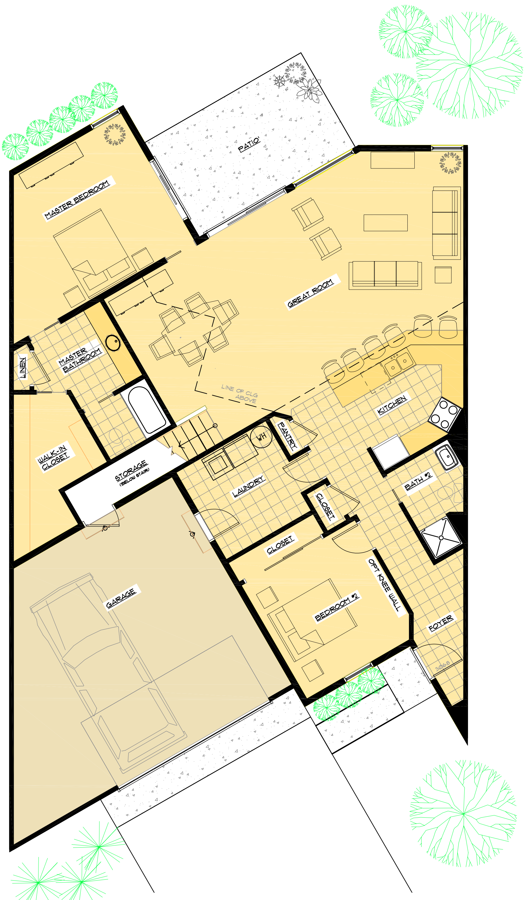
MAIN LEVEL PLAN
